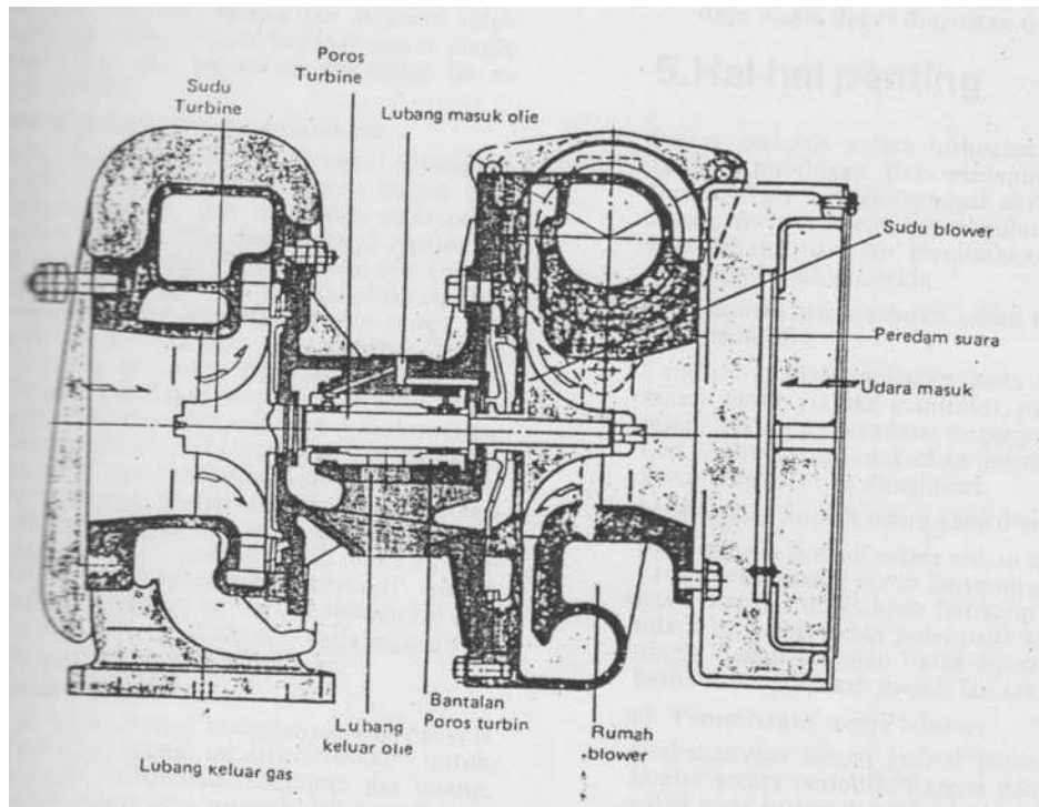
Gambar 19. Radial turbocharger.
